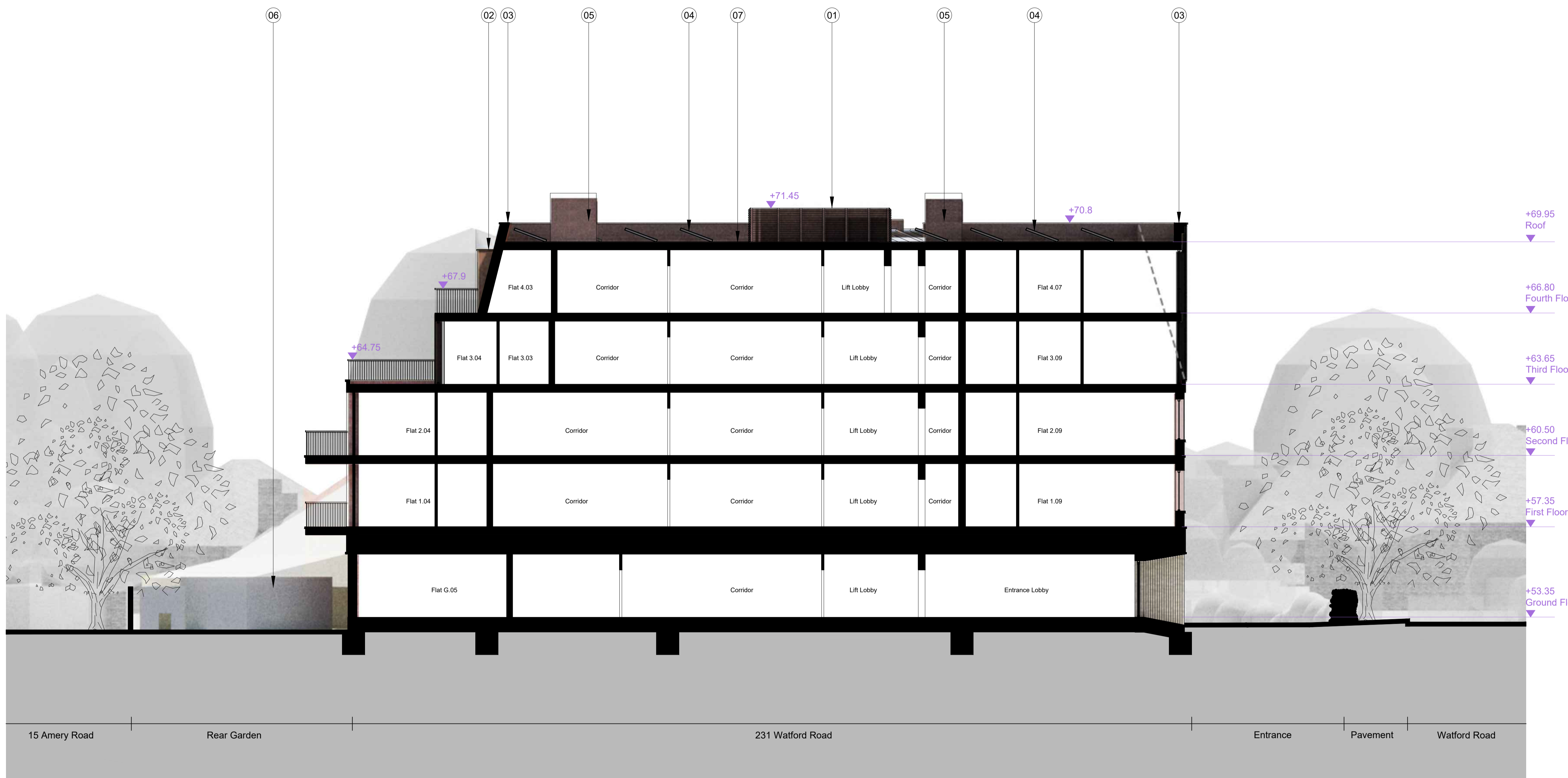
01 Proposed Section A 20.251 1:100@A1, 1:200@A3
